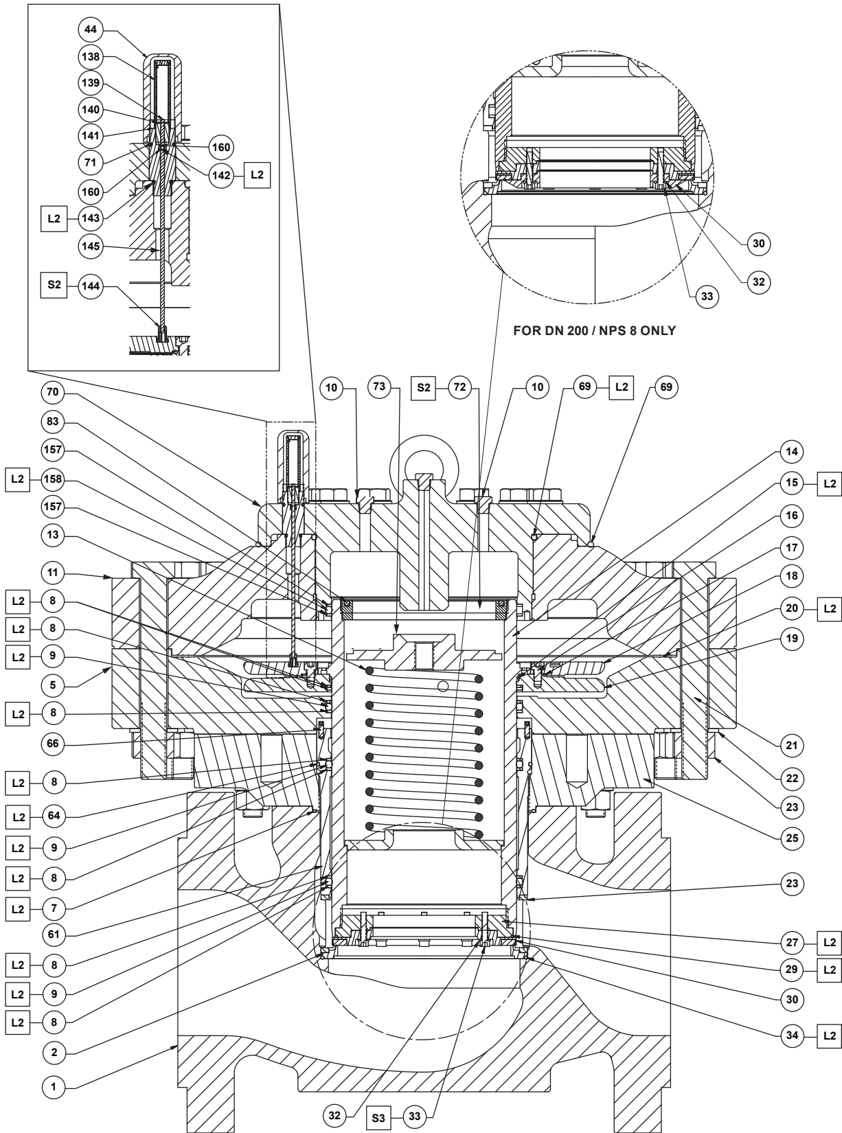
DN 150, 200, 300 X 150 / NPS 6, 8, 12 X 6
